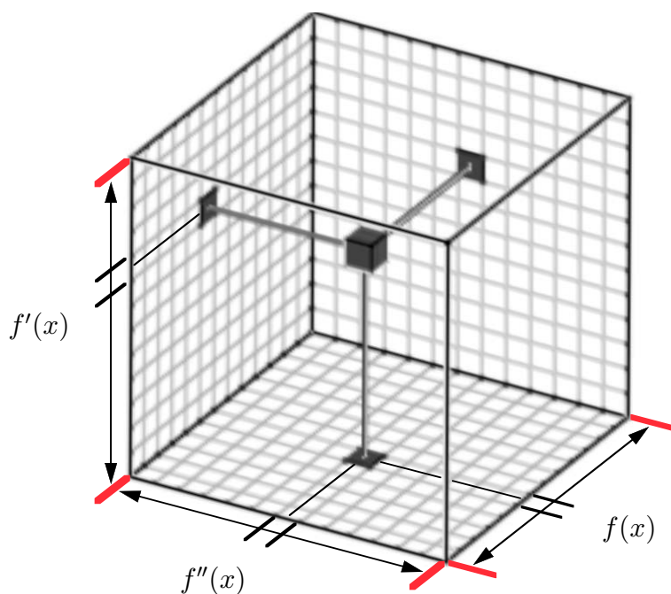
Figure 4.1: Histogram volume structure. Each of the three axes (for f , f' , and f'' ) are divided into bins; the volume is thereby divided into a three dimensional histogram.
