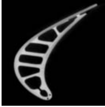
Figure 6.4: Cross-section of blade showing struts
