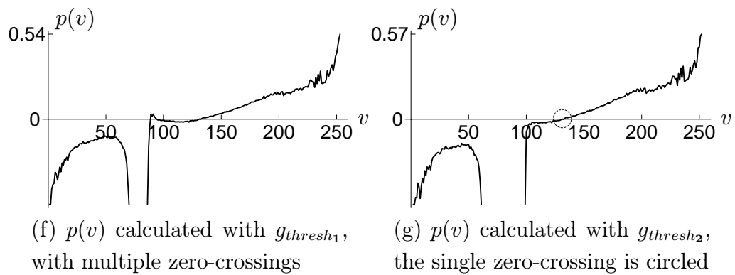
Figure 6.14: Analysis of hippocampal neuron dataset
